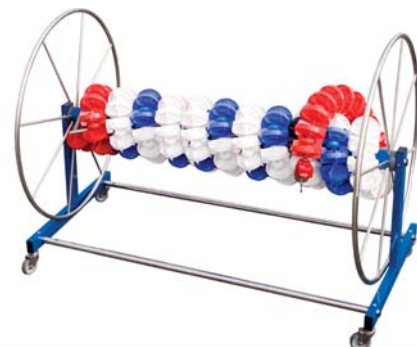
14211 Storage Trolley Malmsten Capacity: 200m Malmsten Standard Racing Lanes. (One field of play) Measurement 2460x1250x1410mm
